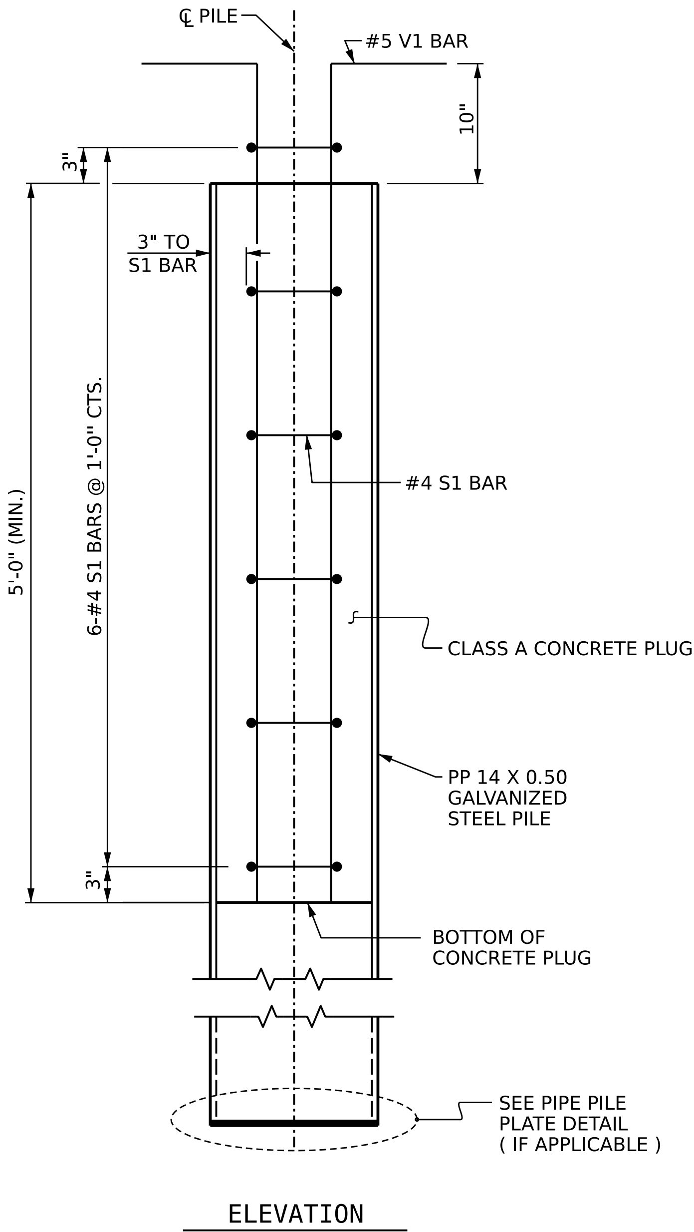
PP 14 X 0.50 GALVANIZED STEEL PILE ( OPEN OR CLOSED END )
