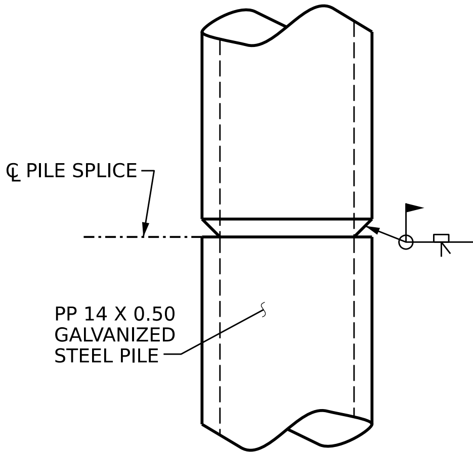
PIPE PILE SPLICE DETAIL
